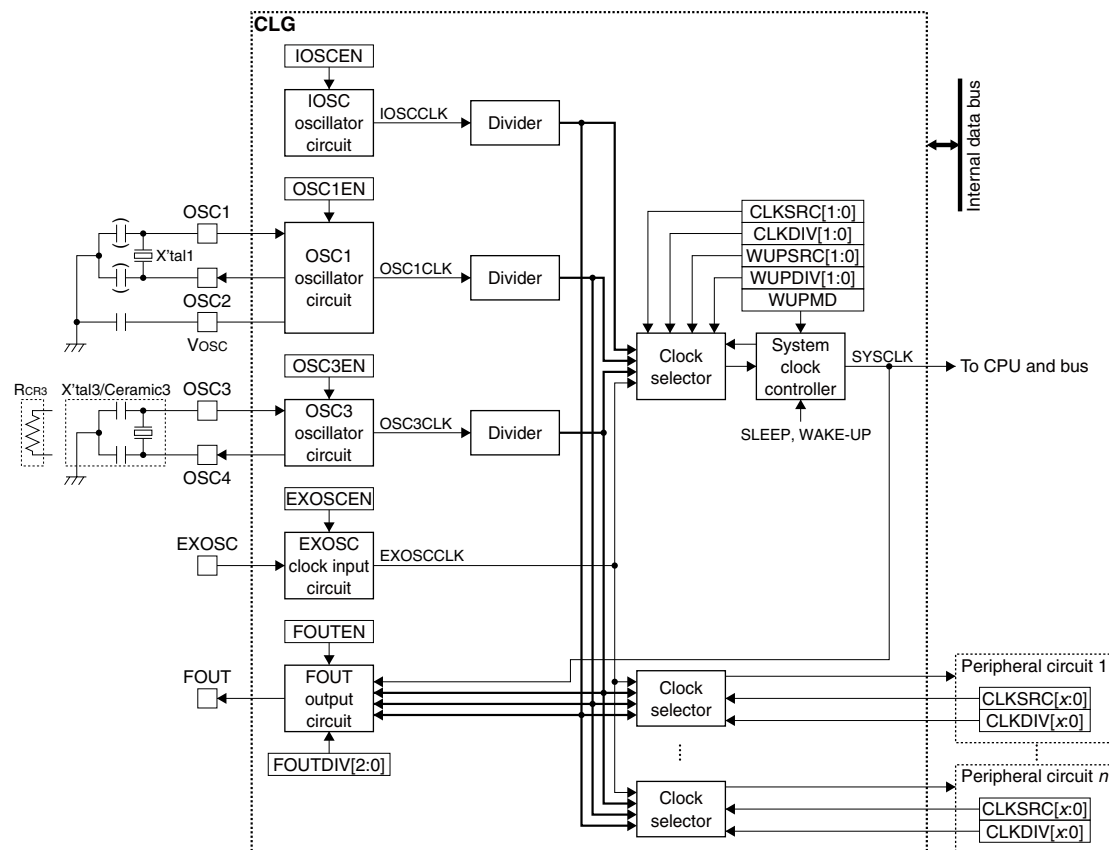
Figure 2.3.1.1 CLG Configuration
