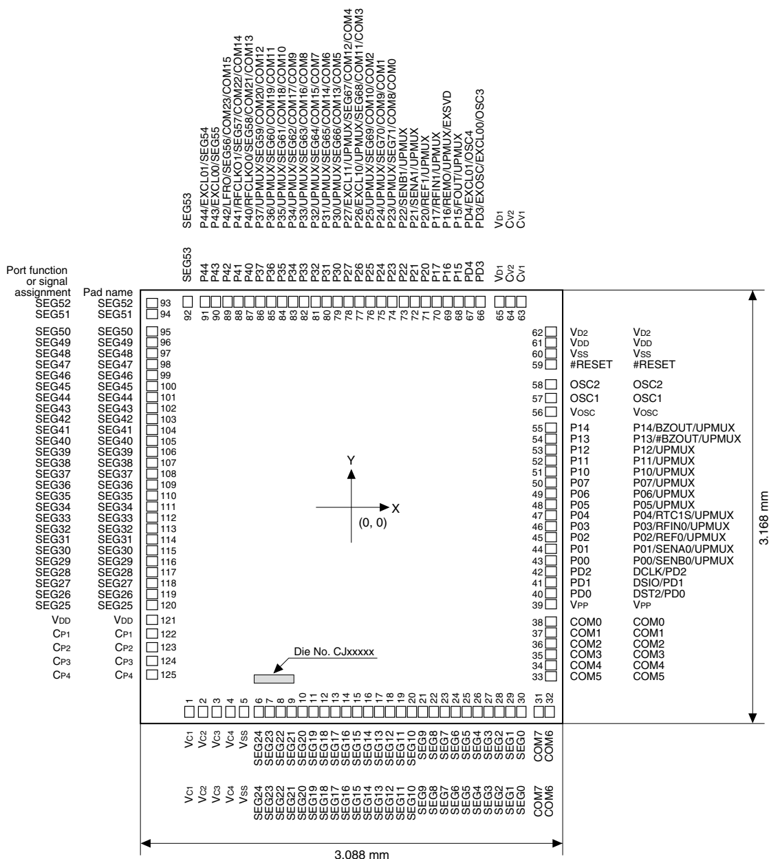
Figure 1.3.2.1 S1C17W22 Pad Configuration Diagram (Chip)
