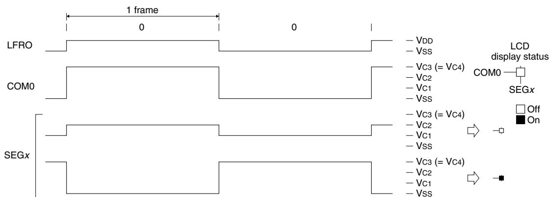
Figure 18.5.5.4 Static Drive Waveform (1/3 bias)
