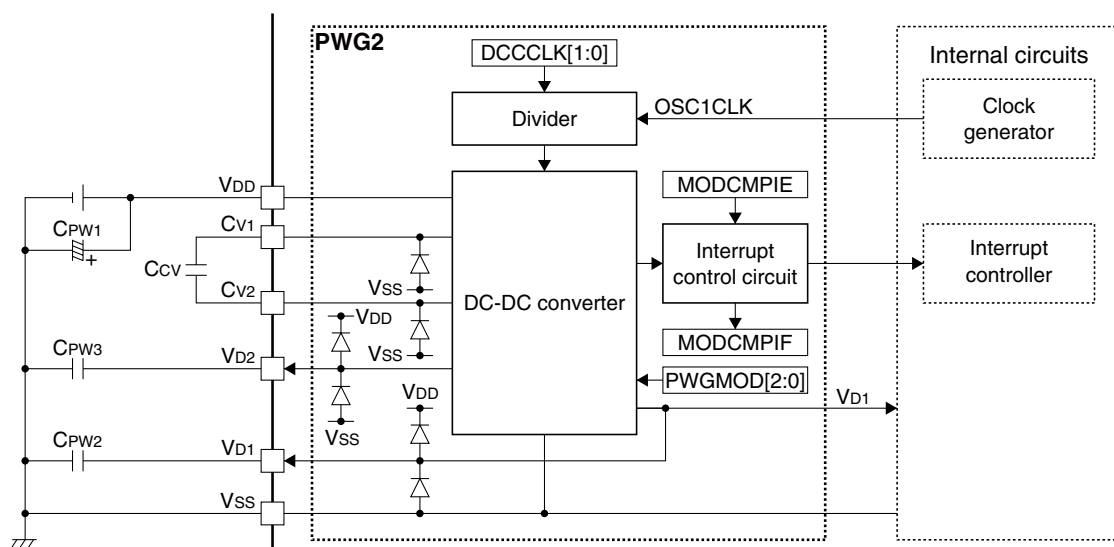
Figure 2.1.1.1 PWG2 Configuration
