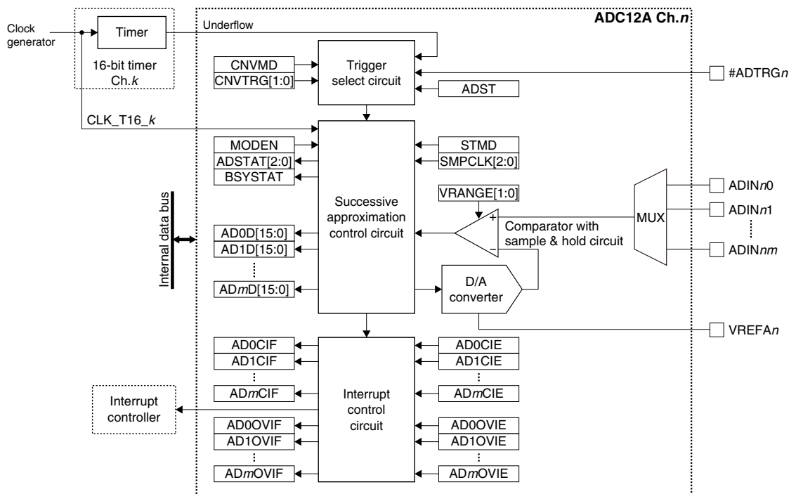
Figure 20.1.1 ADC12A Configuration
