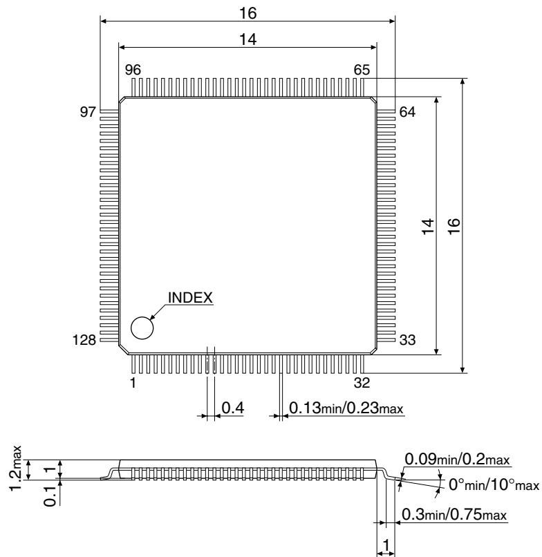
Figure 25.1 TQFP15-128pin Package Dimensions
