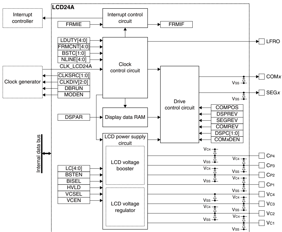
Figure 18.1.1 LCD24A Configuration
