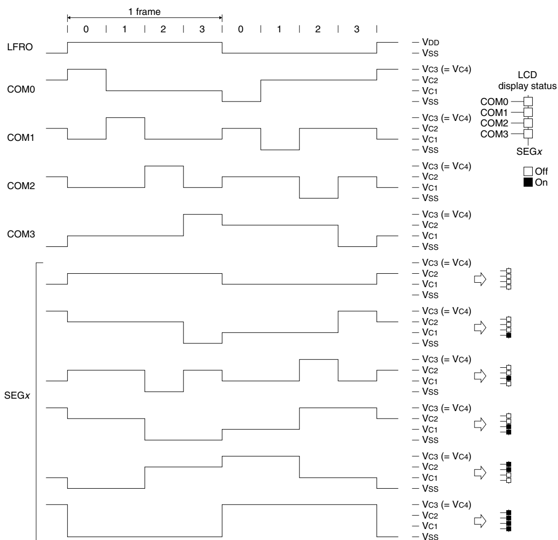
Figure 18.5.5.3 1/4 Duty Drive Waveform (1/3 bias)
