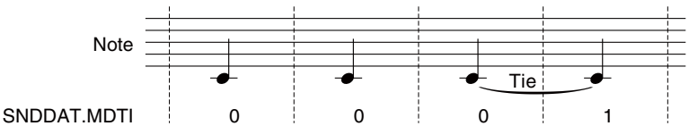
Figure 16.4.4.2 Tie
