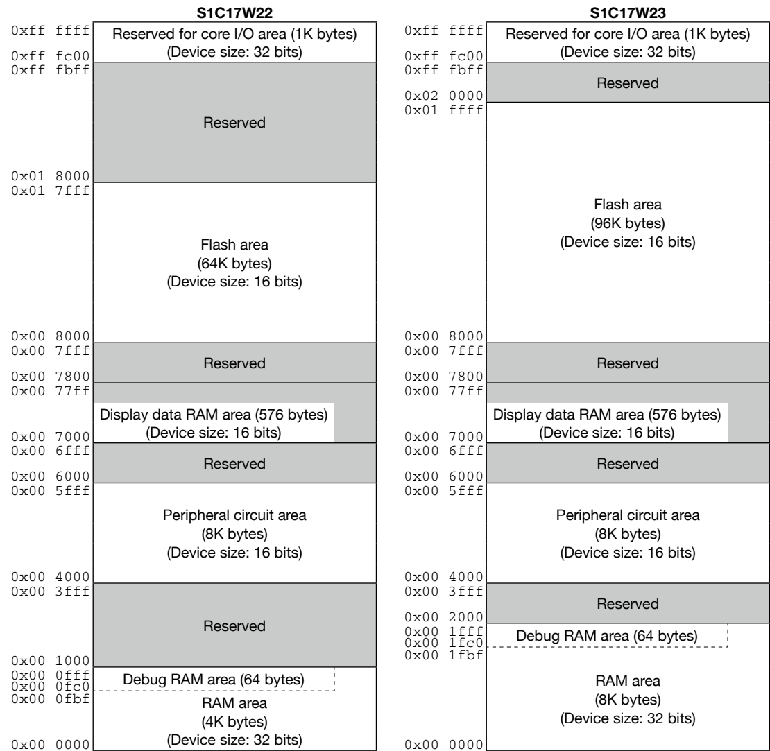
Figure 4.1.1 Memory Map
