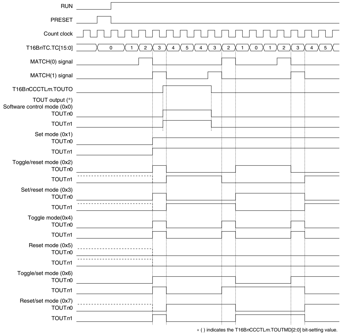
Figure 15.4.4.3 TOUT Output Waveform (T16BnCCCTL0.TOUTMT bit = 1, T16BnCCCTL1.TOUTMT bit = 0)
