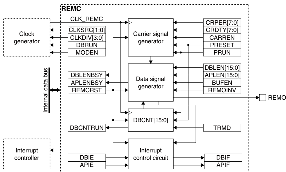
Figure 17.1.1 REMC Configuration
