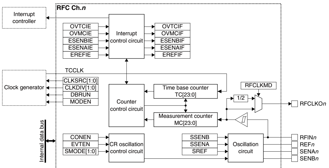
Figure 19.1.1 RFC Configuration
