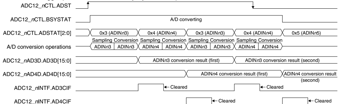
Figure 20.4.4.1 A/D Conversion Operations
