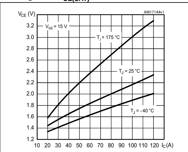
Figure 7. V_{CE(SAT)} vs. collector current
