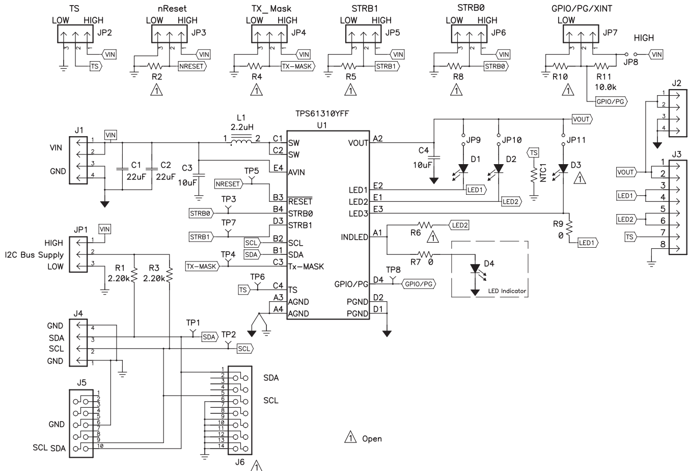
Figure 15. TPS61310EVM-638 Schematic
