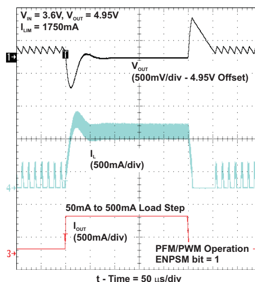
Figure 9. Load Transient
