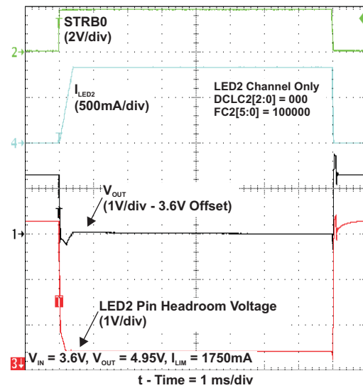
Figure 5. Flash Sequence
