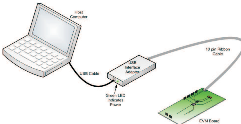
Figure 1. USB Interface Adapter Connection
