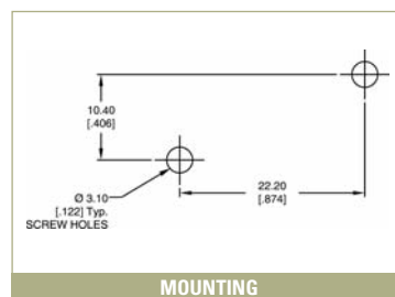
MOUNTING
