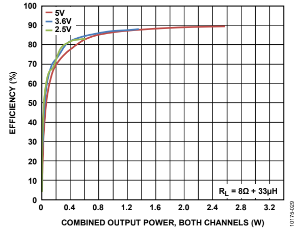
Figure 22. Efficiency vs. Output Power into 8Ω
