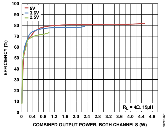
Figure 19. Efficiency vs. Output Power into 4Ω
