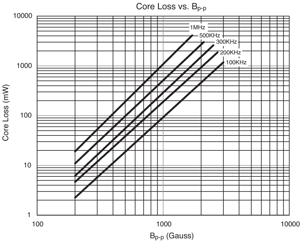
Core loss
