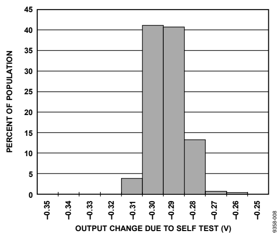
Figure 6. X-Axis Self-Test Response at 25°C, V_S = 3\text{ V}
