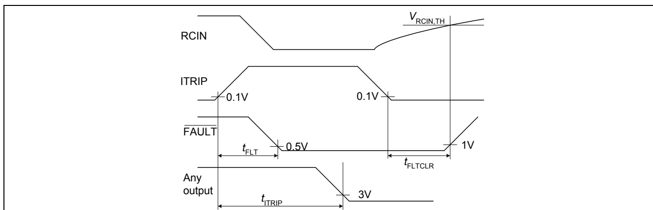
Figure 17 ITRIP-Timing
