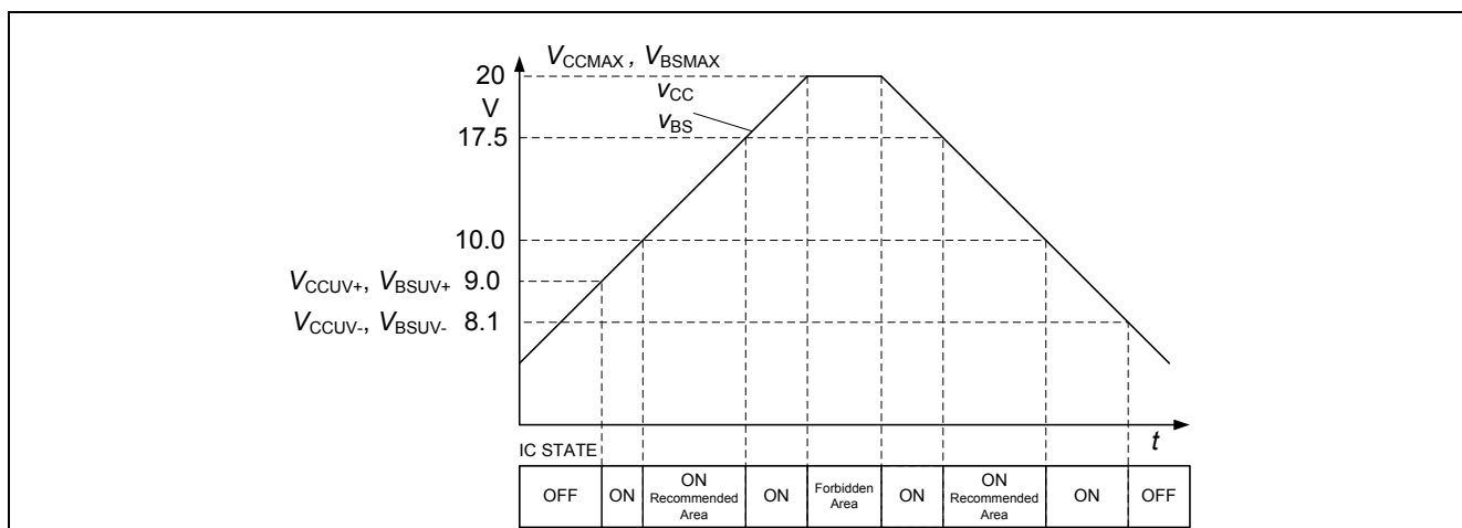
Figure 16 Operating Areas (6EDL04N06PC)
