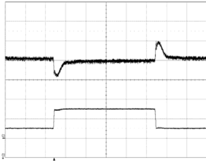
Output voltage response to load current step- change (9.5 – 28.5 – 9.5 A) at: T_{ref} = +25^{\circ}\text{C} , V_I = 53\text{ V} , C_o = 3.8\text{ mF}
