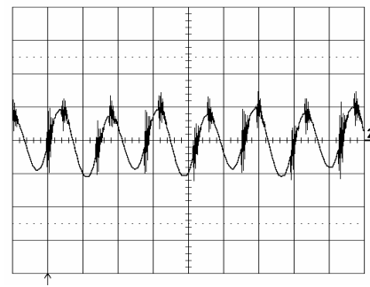
Output voltage ripple at: T_{ref} = +25^{\circ}\text{C} , V_I = 53\text{ V} , I_O = 20\text{ A} resistive load. Trace: output voltage (20 mV/div.). Time scale: (2 µs/div.).
