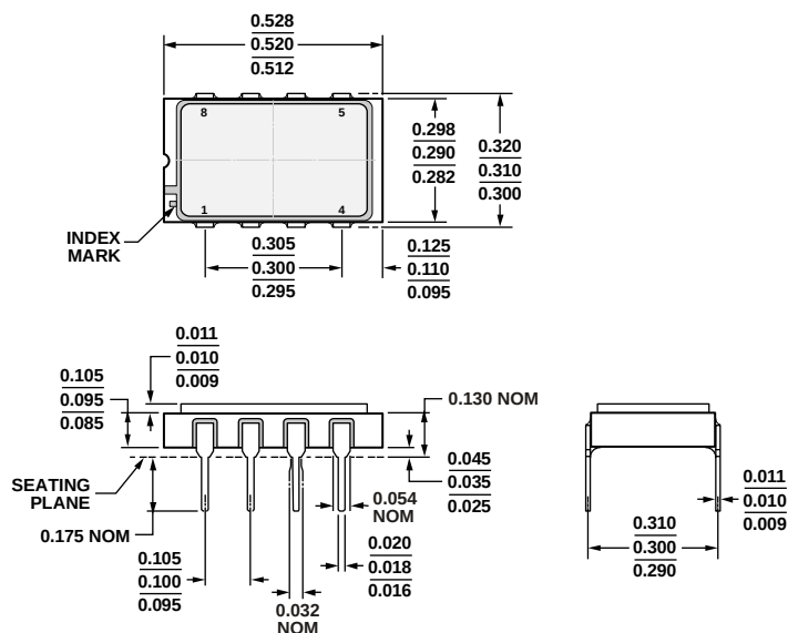
Figure 20. 8-Lead Side-Brazed Ceramic Dual In-Line Package [SBDIP] (D-8-1)
