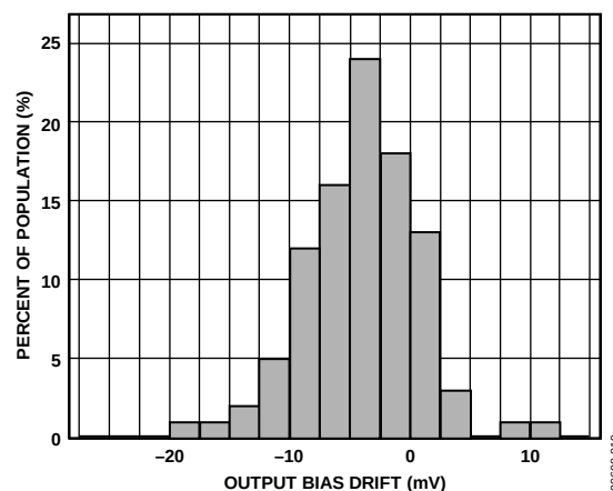
Figure 18. Y-Axis Zero g Output Bias Drift over 1000 Hours at T_A = 175^\circ\text{C} , Powered
