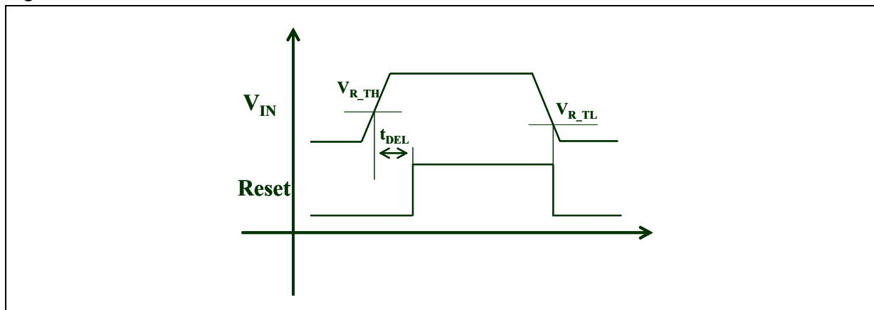
Figure 12. Reset function
