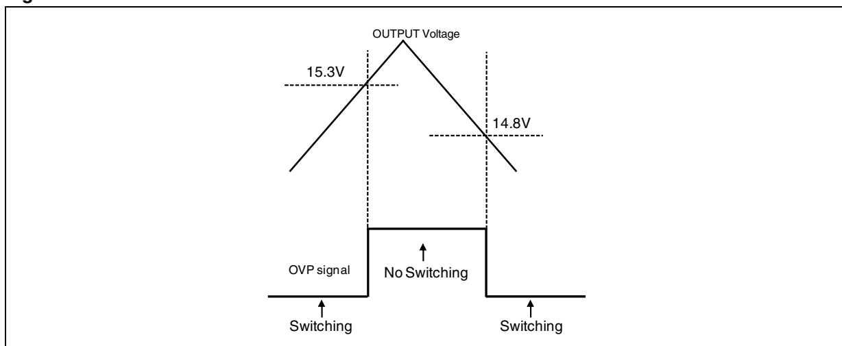
Figure 13. OVP function
