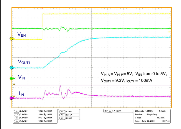
Figure 32. Inrush current
