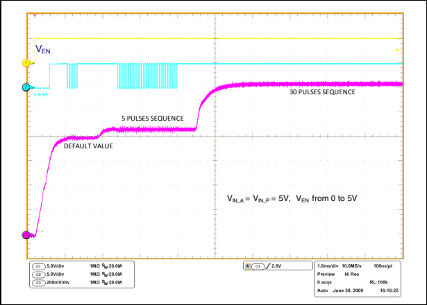
Figure 33. S-Wire protocol
