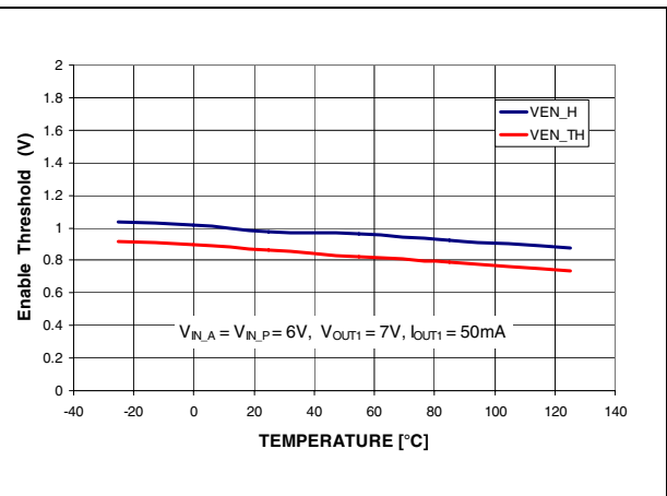
Figure 25. Enable vs. temperature
