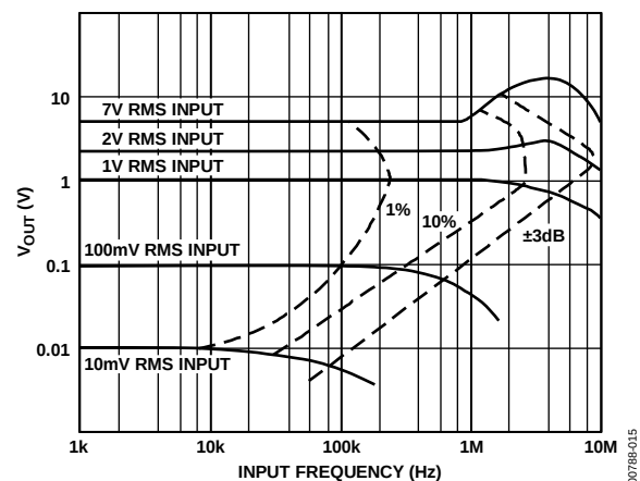
Figure 15. Frequency Response
