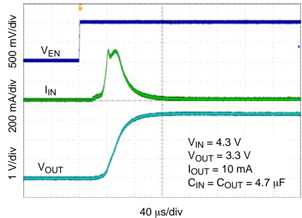
Figure 33. Enable Turn-on Response – V_{OUT} = 3.3\text{ V} , C_{OUT} = 4.7\text{ }\mu\text{F}
