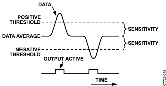
Figure 37. Threshold Sensitivity
