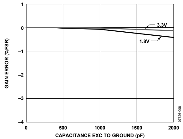
Figure 8. Capacitance Input Gain Error vs. Capacitance EXC to GND, V_{DD} = 1.8\text{ V} and 3.3\text{ V} , CIN to EXC = 3\text{ pF}
