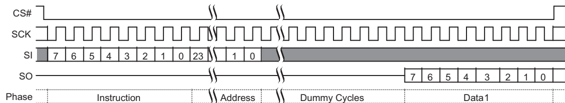
Figure 8.29 Read SFDP Register Command Sequence
