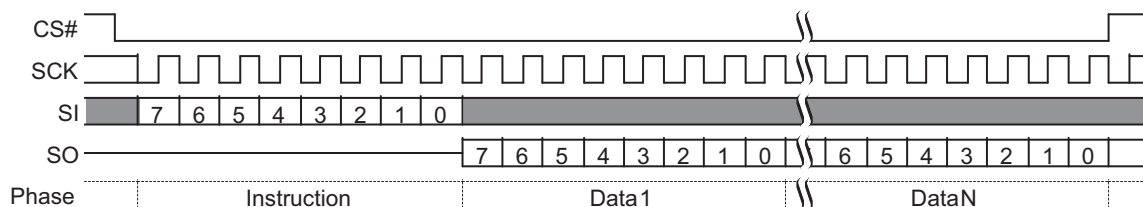
Figure 8.28 Read JEDEC ID Command Sequence
