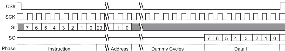
Figure 3.6 Single Bit Wide I/O Command with Latency
