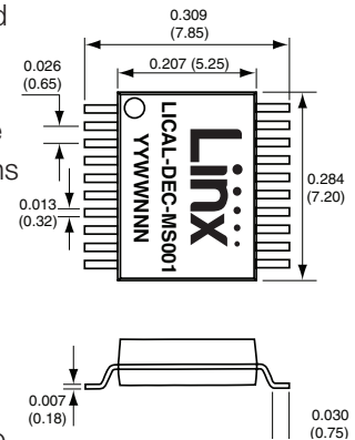
Figure 1: Package Dimensions
