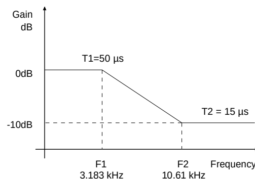
Figure 11. De-Emphasis Curve
