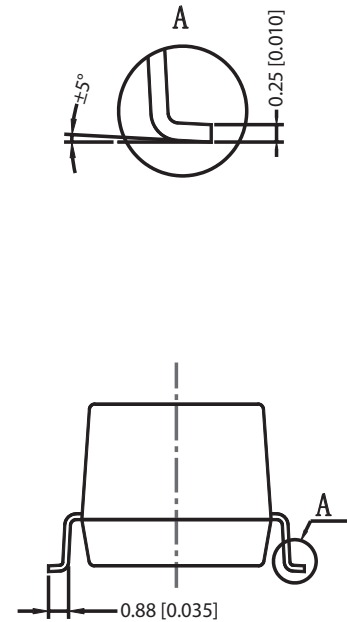
Right View
