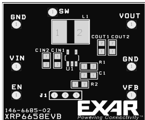
Fig. 3: Component Placement – Top Side
