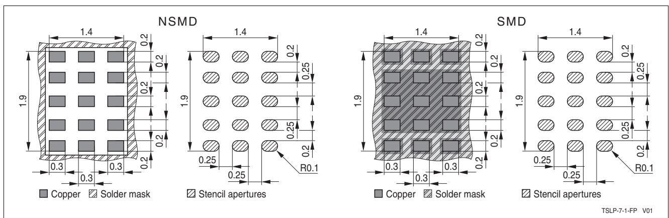
Figure 9-2 Footprint
