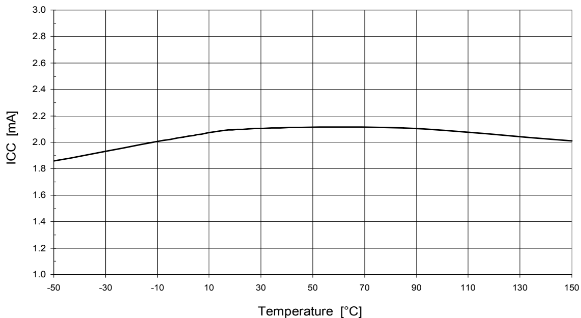
Figure 8-4 I_{CC} as a Function of Temperature, V_{Ctrl} = V_{CC} = 3\text{ V} , R_{ext} = open
