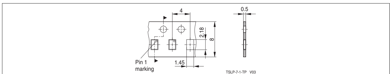
Figure 9-4 Tape Dimensions
