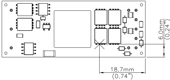
Figure 20: Temperature measurement location
