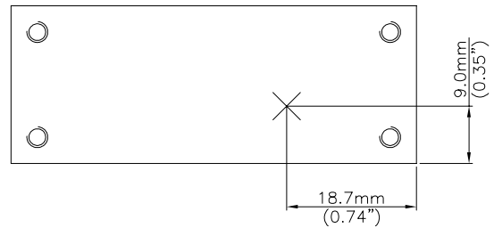
Figure 22: Temperature measurement location
