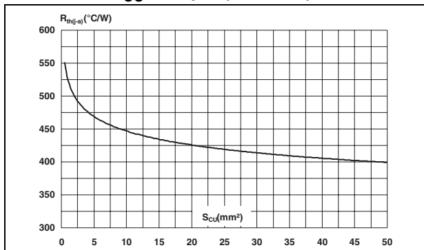
Figure 11. Thermal resistance junction to ambient versus copper surface under each lead, epoxy FR4, e_{CU} = 35 \mu\text{m} (SOD-323)
