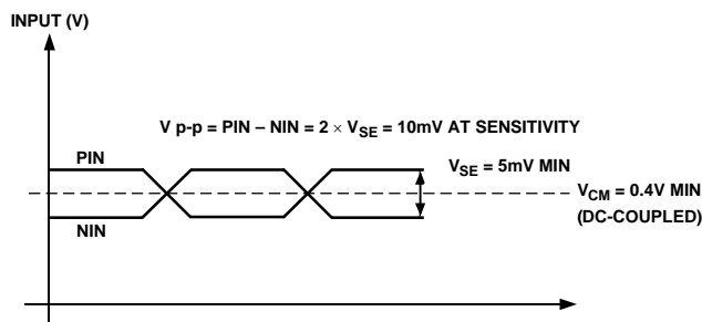
Figure 24. Minimum Allowed DC-Coupled Input Levels
