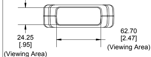
Bottom End View of Assembly
