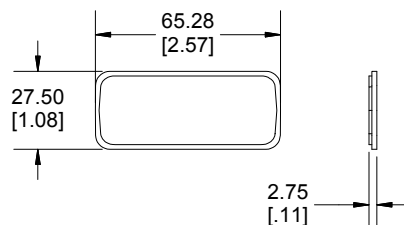
Front/Rear Panel
