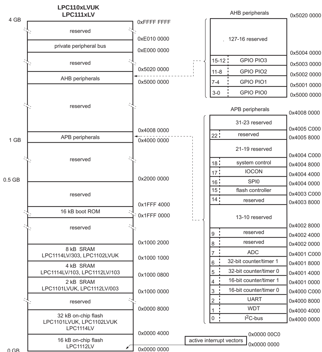
Fig 5. LPC111xLV/LPC11xxLVUK memory map
