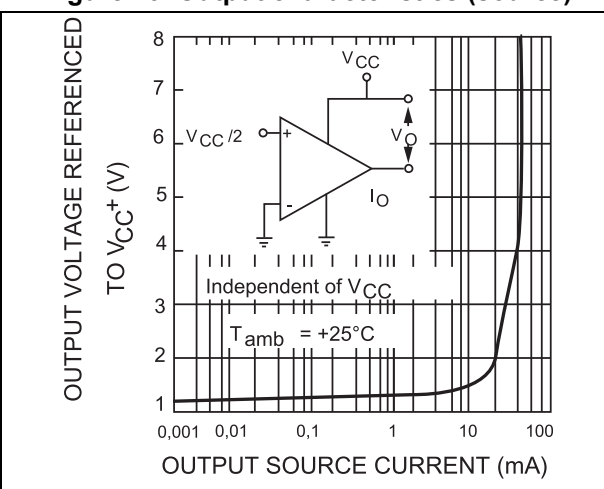
Figure 13. Output characteristics (source)
