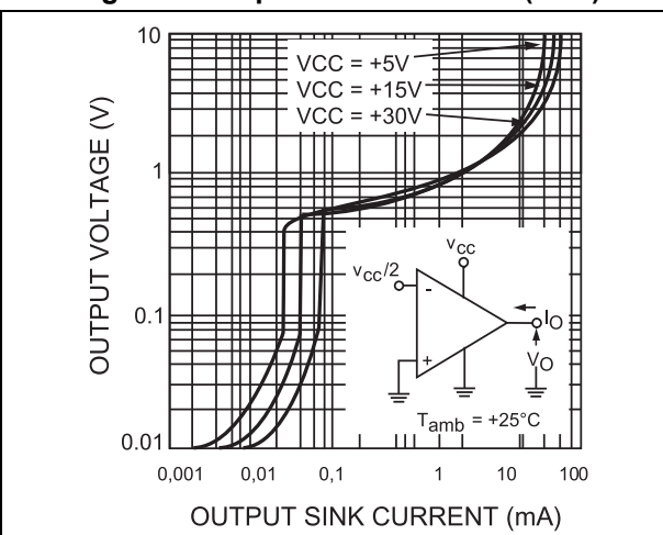
Figure 9. Output characteristics (sink)
