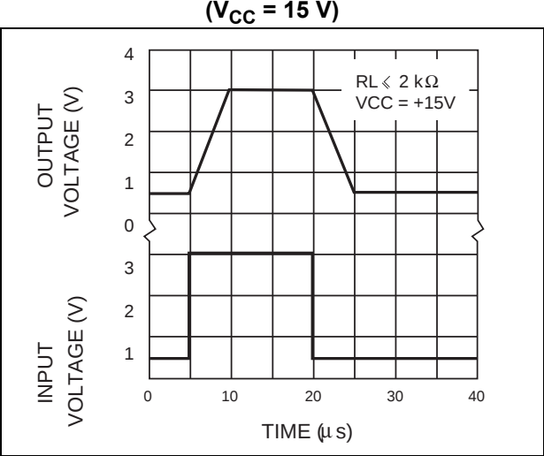
Figure 7. Voltage follower pulse response ( V_{CC} = 15 V)
