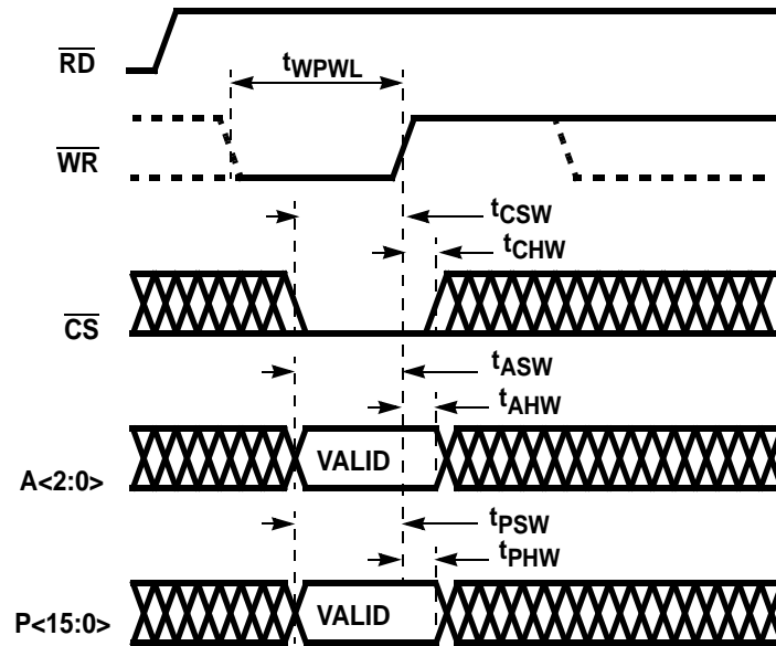
FIGURE 13. MICROPROCESSOR WRITE TIMING ( \mu\text{P mode} = 0 )
