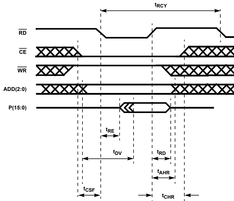
FIGURE 14. MICROPROCESSOR READ TIMING ( \mu\text{P mode} = 0 )
