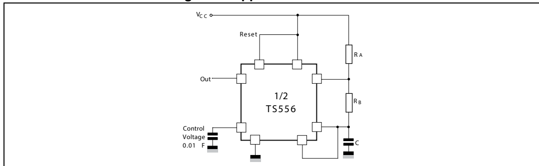
Figure 6. Application schematic
