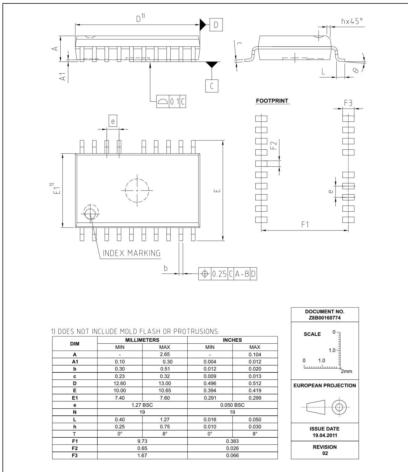
Figure 9 PG-DSO-19-4
