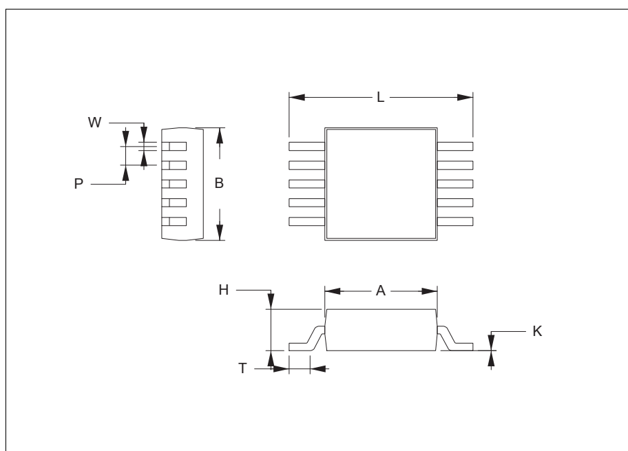
Figure 13.1: MSOP10 Package.
