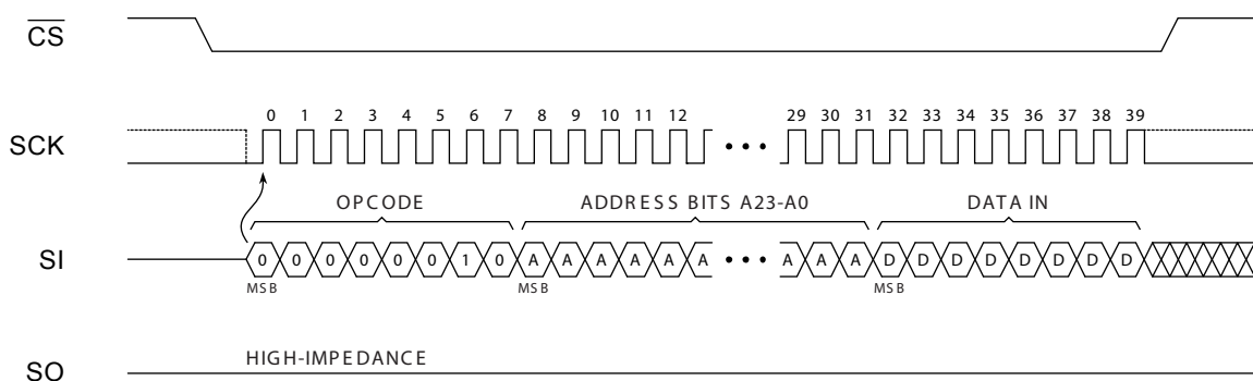
Figure 7-2. Page Program
