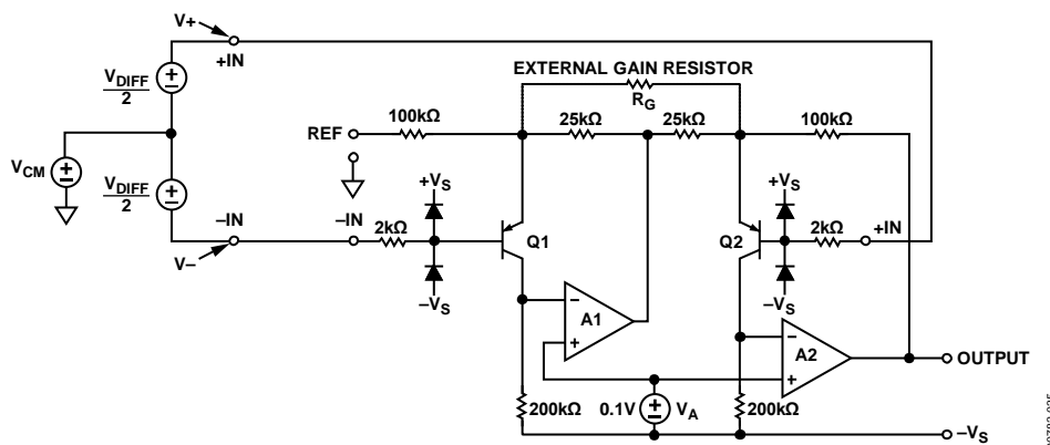
Figure 37. Amplifying Differential Signals with a Common-Mode Component
