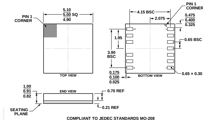
Figure 23. 13-Terminal Land Grid Array [LGA] (CC-13-1) Dimensions shown in millimeters
