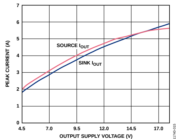
Figure 15. Typical Peak Output Current vs. Output Supply Voltage, 1.2\text{ }\Omega Series Resistance
