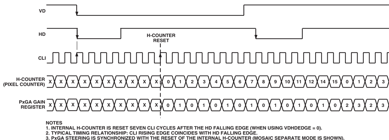
Figure 13. H-Counter Synchronization
