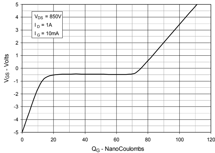
Fig. 15. Gate Charge
