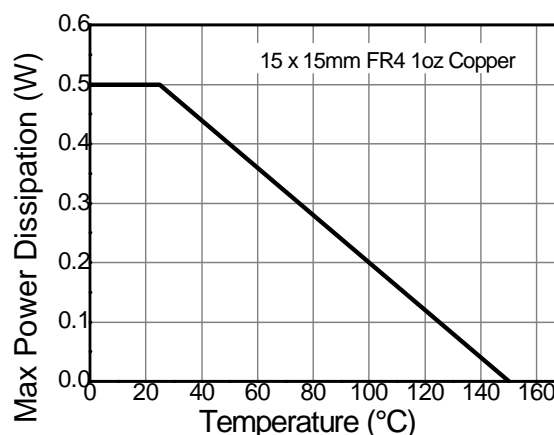
Derating Curve
