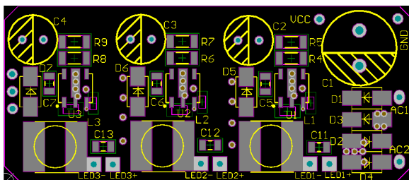
Figure 4 Component Placement Guide -Top Layer
