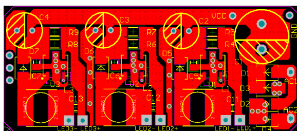
Figure 2 PCB Layout-Top Layer
