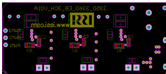
Figure 5 Component Placement Guide -Bottom Layer
