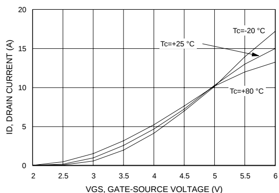
Figure 13. Drain current vs gate-source voltage
