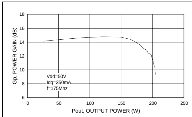
Figure 10. Power gain vs output power
