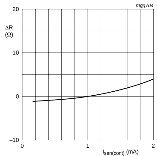
Fig 1. Sensor resistance as a function of operating current
