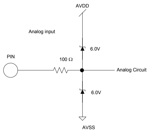
Figure 21 Analog input
