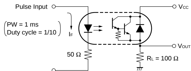
*1 Test circuit for switching time
