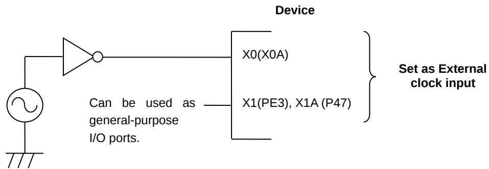
Example of Using an External Clock
