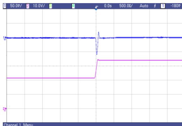
Fig. 35 AVO75-48S2V5 typical transient response to step increase in load from 50% to 75% of full load, room temperature, 48Vdc input ( \Delta I_o/\Delta t=0.1A/1\mu s )
