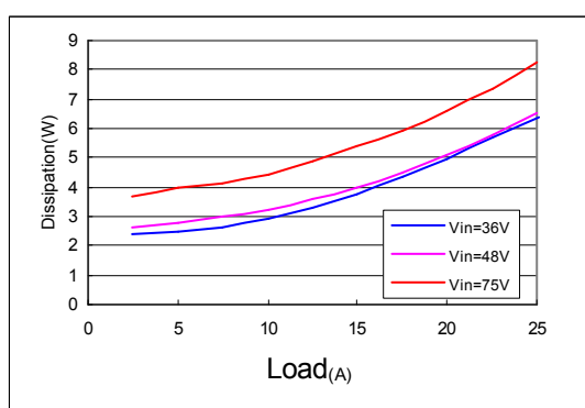
Fig. 18 Typical power dissipation of AVO75-48S2V5
