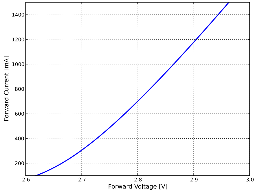
Figure 9. Typical forward current vs. forward voltage, L1T2-xyyy0000000000.
