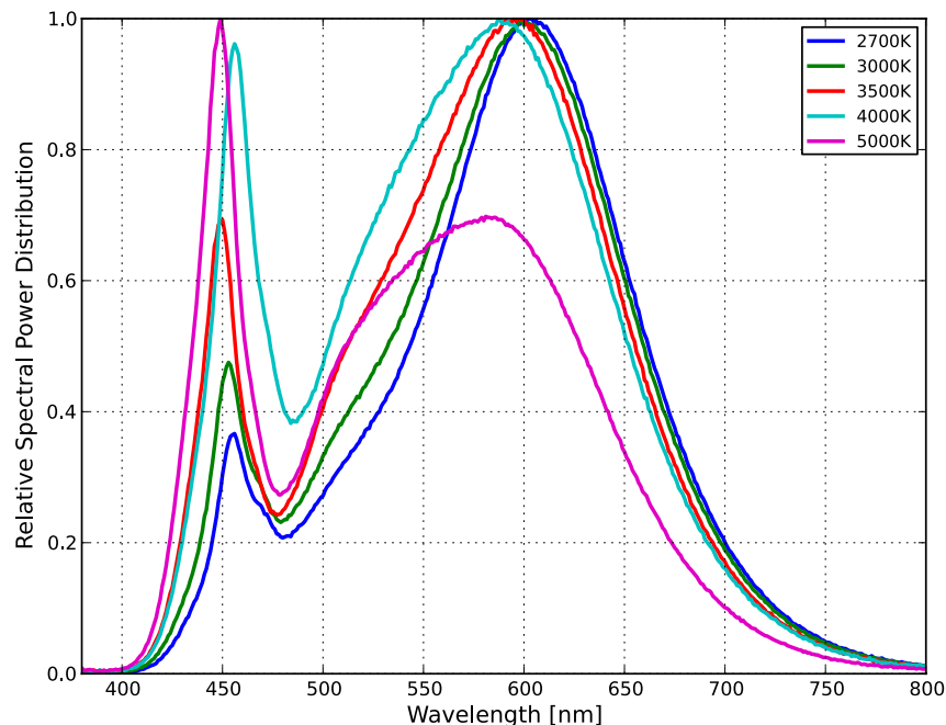
Figure 5. Color Spectrum of L1T2-xx800000000000.
