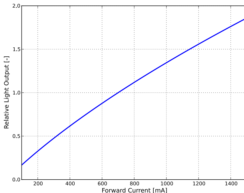
Figure 8. Typical relative luminous flux vs. forward current, L1T2-xyyy0000000000.
