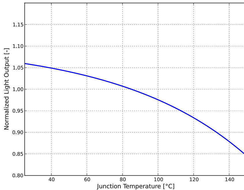
Figure 7. Typical relative light output vs. junction temperature, L1T2-xyyy0000000000.
