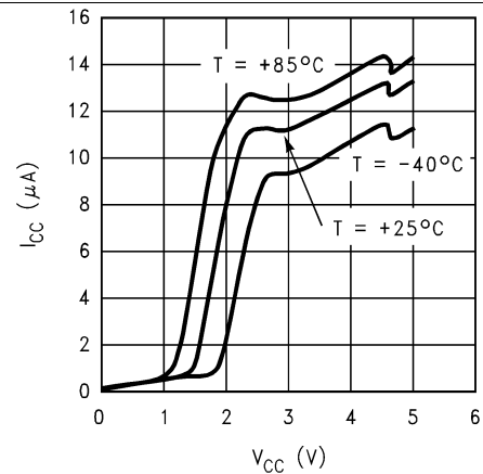
Figure 2. I_{CC} vs V_{CC}
