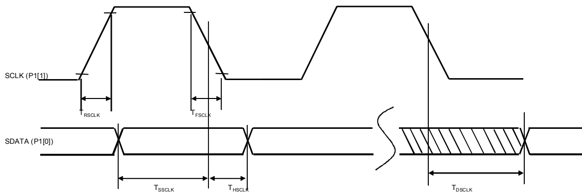
Figure 9. AC Waveform
