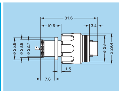
FG●LM.U2A.XPAT Straight plug, key (W) or key (R) with arctic grip and mold stop
