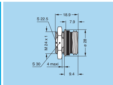
EG●LM.U2A.XPL Fixed socket, nut fixing, key (W) or key (R)
