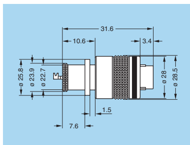
FM●LM.U2A.XPAT Straight plug, key (W) or key (R) with knurled grip and mold stop
