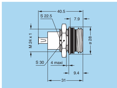
EG●LM.U2A.XPP Fixed socket, female to female, nut fixing, key (W) or key (R)
