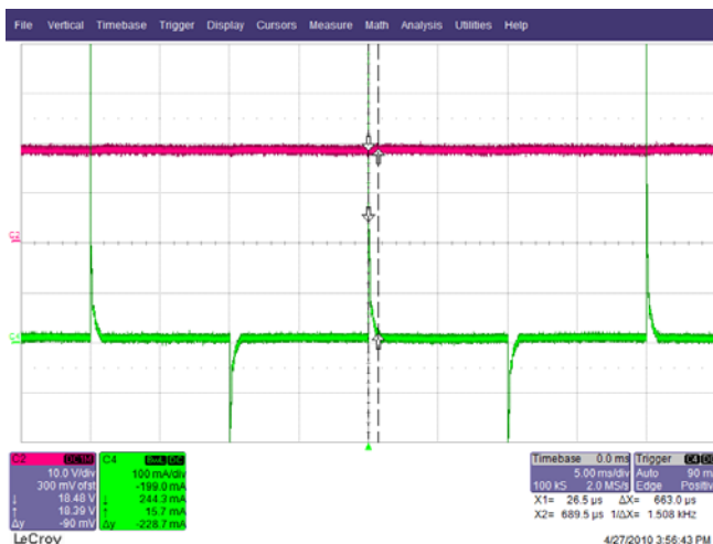
Figure 37 – 230 VAC, 12° Phase. Upper: V_{OUT} , 10 V / div. Lower: I_{IN} , 0.1 A / div., 5 ms / div.
