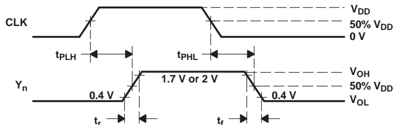
Figure 3. Voltage Waveforms Propagation Delay Times
