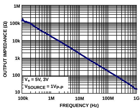
FIGURE 6. DISABLED OUTPUT IMPEDANCE vs FREQUENCY
